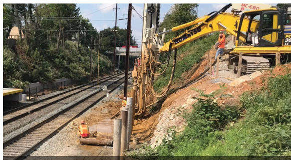
Micropiles - Mount Joy Train Station, Mount Joy, Pa.
